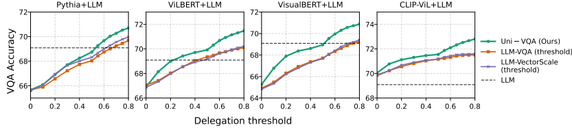
Figure 6: Performance comparison of the proposed method against LLM-VQA, and LLM-VectorScale (threshold), with respect to the delegation threshold. Accuracy at zero delegation is accuracy of TS-VQA model.
