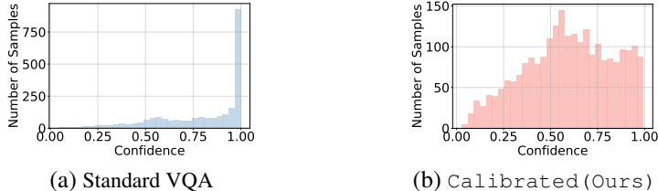
Figure 16: Confidence histograms for correct predictions on AdVQA (OOD; trained on VQA-v2): (a) Standard VQA and (b) Calibrated (ours).
