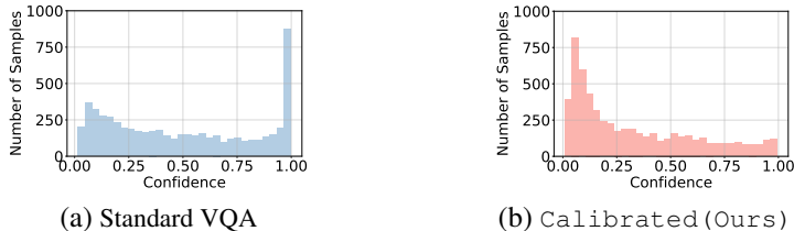
Figure 15: Confidence histograms for incorrect predictions on AdVQA (OOD; trained on VQA-v2): (a) Standard VQA and (b) Calibrated (ours).
